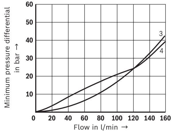
\Delta p_{min} \cdot q_V characteristic curves – Version "B" and "P"
