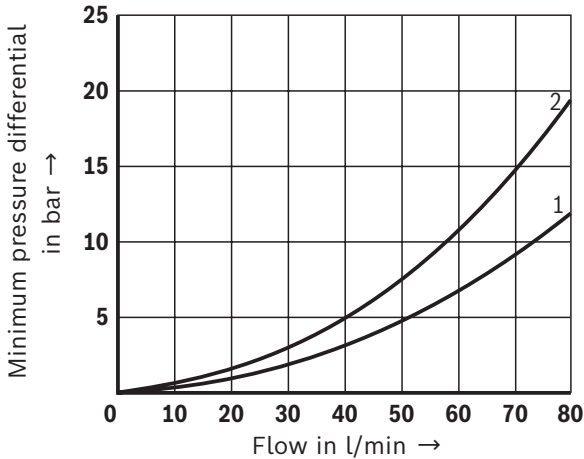
\Delta p_{min} \cdot q_V characteristic curves – Version "A"
