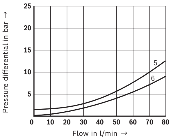
\Delta p \cdot q_V characteristic curves – Version "A"
