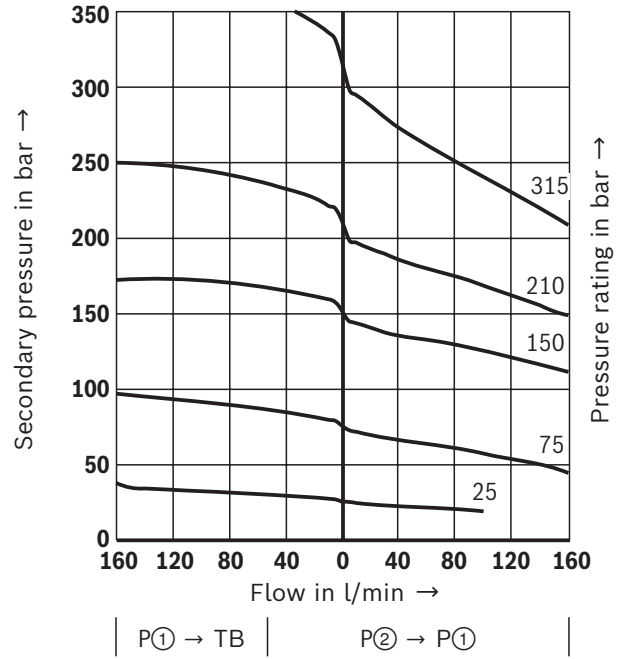
p_A \cdot q_V characteristic curves – Version "B" and "P"
