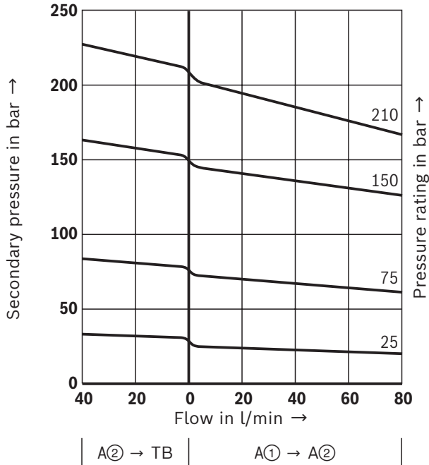
p_A \cdot q_V characteristic curves – Version "A"
